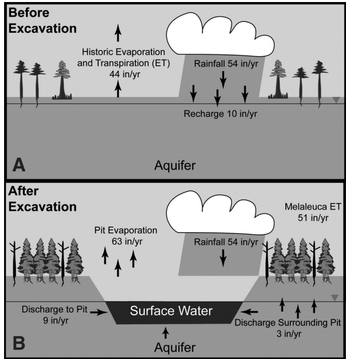
Figure 2. Permanent reduction of groundwater resources by excavations, based on historic rainfall, evapotranspiration (ET), and evaporation (E) rates for southern Florida (Chin, 1996; Krulikas and Giese, 1995; Odum, 1984; USACE, 2000; printed with permission). (A) Before excavation, historic rainfall and ET are ~137 cm/yr (reported as 54 in/yr) and ~112 cm/yr (reported as 44 in/yr), respectively, resulting in net recharge to the aquifer system of ~25 cm/yr (10 in/yr). (B) After excavation, historic rainfall is held constant, while ET over the excavated pit is converted to E, with an increase to ~160 cm/yr (reported as 63 in/yr), and ET surrounding the pit increases to ~130 cm/yr (reported as 51 in/yr), due to induced conversion from water-conserving to water-depleting vegetative cover, such as invasive and alien species, permanently lowering the water table (▼). See text for details.
